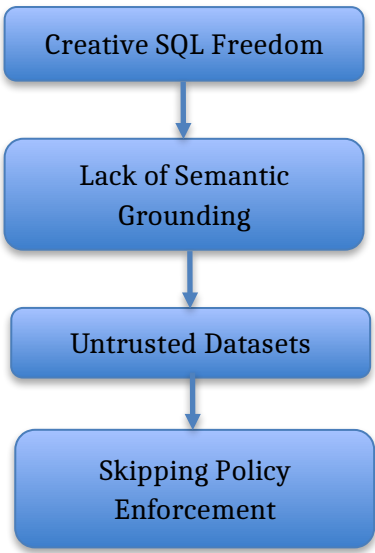
Figure 3: NL-to-SQL Challenges
